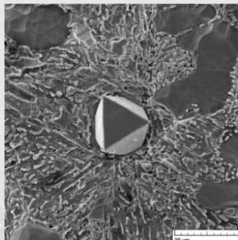
Primary \beta -Si plates surrounded by dendrites of primary \alpha -Al and modified eutectic ( \alpha -Al + \beta -Si) developed during solidification of eutectic AlSi12 alloy
